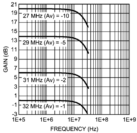
Gain vs Frequency R_F = 3k\Omega, V_S = \pm 15V
